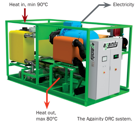
The Againty ORC system. Model AT200.
